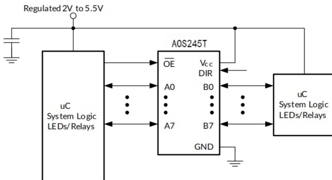
Figure 2. Application Schematic
