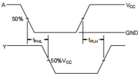
Figure 3. Switching Waveform
